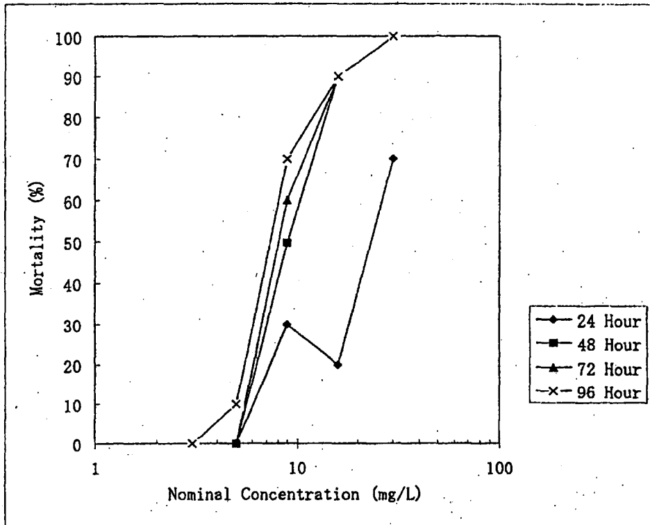
Figure 1 Concentration-Response Curve
