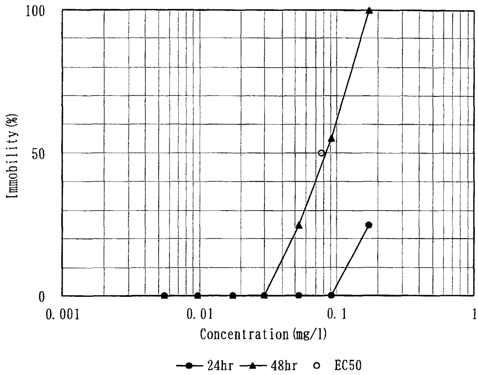
Figure 1. Concentration-immobility curve
