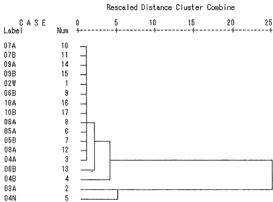
Dendrogram using Average Linkage (Between Groups)
