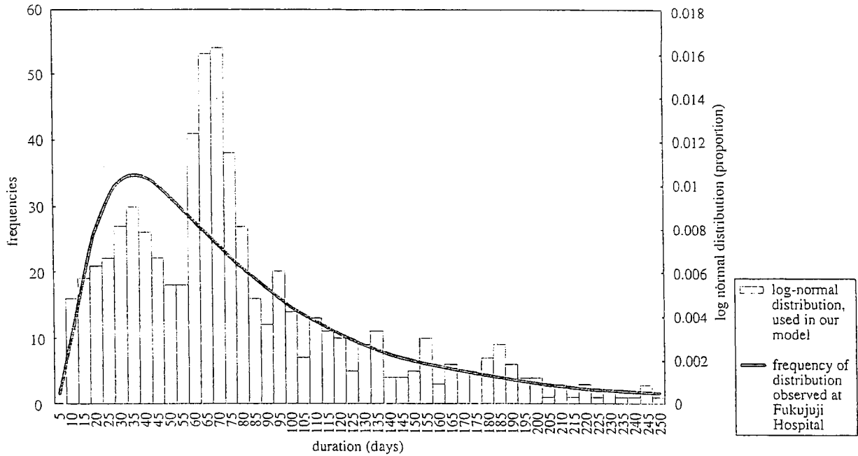
Fig. Distribution of duration of hospitalization at Fukujiji Hospital and log normal distribution used in our model
