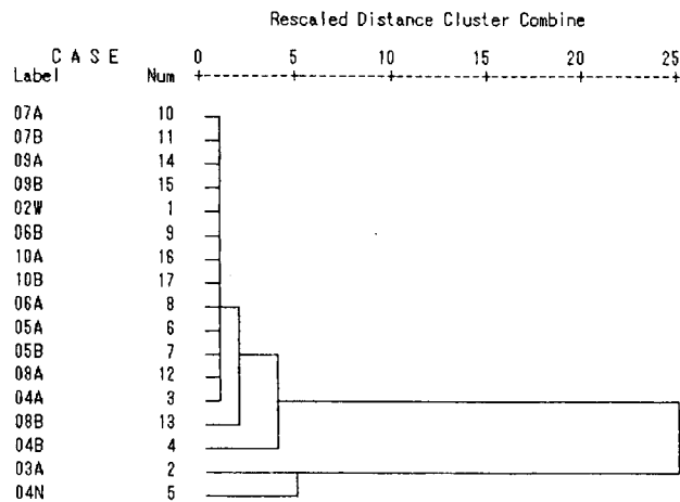
Dendrogram using Average Linkage (Between Groups)
