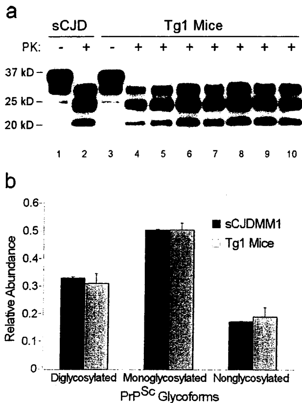
Figure 6. Immunoblots and glycoform ratios of PK-resistant PrP Sc from the sCJDM1 donor and sCJDM1-inoculated Tg1 mice. a , Immunoblot of PrP. PK-untreated (lane 1) PrP and PK-treated (lane 2) PrP were obtained from the sCJDM1 donor; PK-untreated (lane 3) PrP and PK-treated (lanes 4–10) PrP were obtained from the seven sCJDM1-inoculated Tg1 mice. b , Glycoform ratio analysis of PK-resistant PrP Sc . PK-untreated and PK-treated brain homogenates were processed as in Figure 2, but blots were probed with 3F4. Error bars are based on quantitative analyses of digital chemiluminescence images of triplicate Western blots of brain homogenates from a subject with sCJDM1 (the inoculum) and duplicate Western blots of the seven Tg1 mice infected with sCJDM1. kd, Kilodalton.
