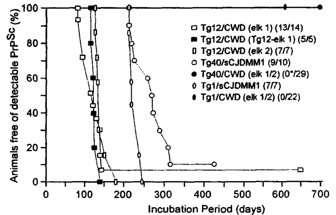
Figure 1. Survival curves of humanized and cervidized transgenic mice. Six- to eight-week-old cervidized Tg12 and humanized Tg1 and Tg40 mice were inoculated intracerebrally with 30 \mu l of 1% brain homogenate from two CWD-affected elk or a subject with sCJDMM1. The Tg12 mice were also inoculated with brain homogenates from elk 1 CWD-affected Tg12 mice to evaluate the species barrier of elk CWD transmission to the Tg12 mice. The average incubation times were as follows: 118 \pm 6 d for elk 1 CWD-inoculated Tg12 mice (open squares); 125 \pm 4 d for secondary transmission of elk 1 CWD in Tg12 mice (filled squares); 142 \pm 7 d for elk 2 CWD-inoculated Tg12 mice (open rectangles); 263 \pm 13 d for the sCJDMM1-inoculated Tg40 mice (open circles); and 226 \pm 5 d for the sCJDMM1-inoculated Tg1 mice (open ovals). None of the 29 CWD-inoculated Tg40 mice (filled circle) or the 22 CWD-inoculated Tg1 mice (filled oval) had detectable PK-resistant PrP Sc or substantial histopathology after >756 and >657 dpi, respectively. The asterisk indicates that three Tg40 mice became ataxic between 420 and 509 dpi but were free of prion infection. Parentheses indicate prion-positive mice per total inoculated mice.
