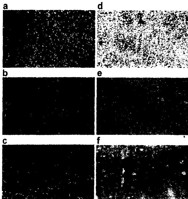
Figure 2. Histopathology, PrP immunohistochemistry, and apoptosis examination in CWD-affected Tg12-cervidized mice. Prominent spongiform degeneration was present in the cerebral cortex (a) along with marked neuronal loss in the granule cell layer of the cerebellum (b) when compared with age-matched control Tg12 mice (c) (hematoxylin and eosin staining; 20× magnification). PrP deposits formed a fine granular pattern interspersed with plaque-like deposits (arrow) in the cerebral cortex (d) and in the granule cell layer of the cerebellum (e) (mAb 8H4; 20× magnification). Neuronal apoptosis (arrow) was present in the granule cells of the hippocampus (f) and in other brain regions (TUNEL; 40× magnification).
