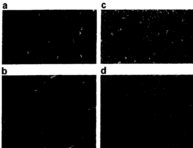
Figure 5. Histopathology and PrP Sc deposition in the brains of sCJDM1-infected Tg40 mice. In the brains of sCJDM1-infected Tg40 mice, hematoxylin and eosin staining revealed moderate spongiform degeneration with fine vacuoles in the cerebral cortex ( a ) accompanied by even milder spongiosis in other brain areas (20× magnification), but the granule cell layer of the cerebellum ( b ) appears mostly intact (40× magnification). Immunohistochemistry for PrP Sc with 3F4 revealed fine PrP Sc deposits in the cerebral cortex ( c ), with more intense PrP Sc deposits in the cerebellum ( d ) (20× magnification).
